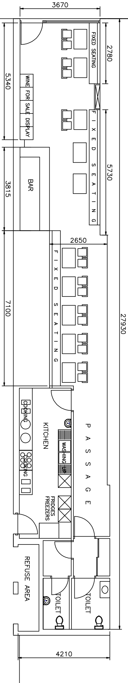
PROPOSED GROUND FLOOR PLAN 1/100
