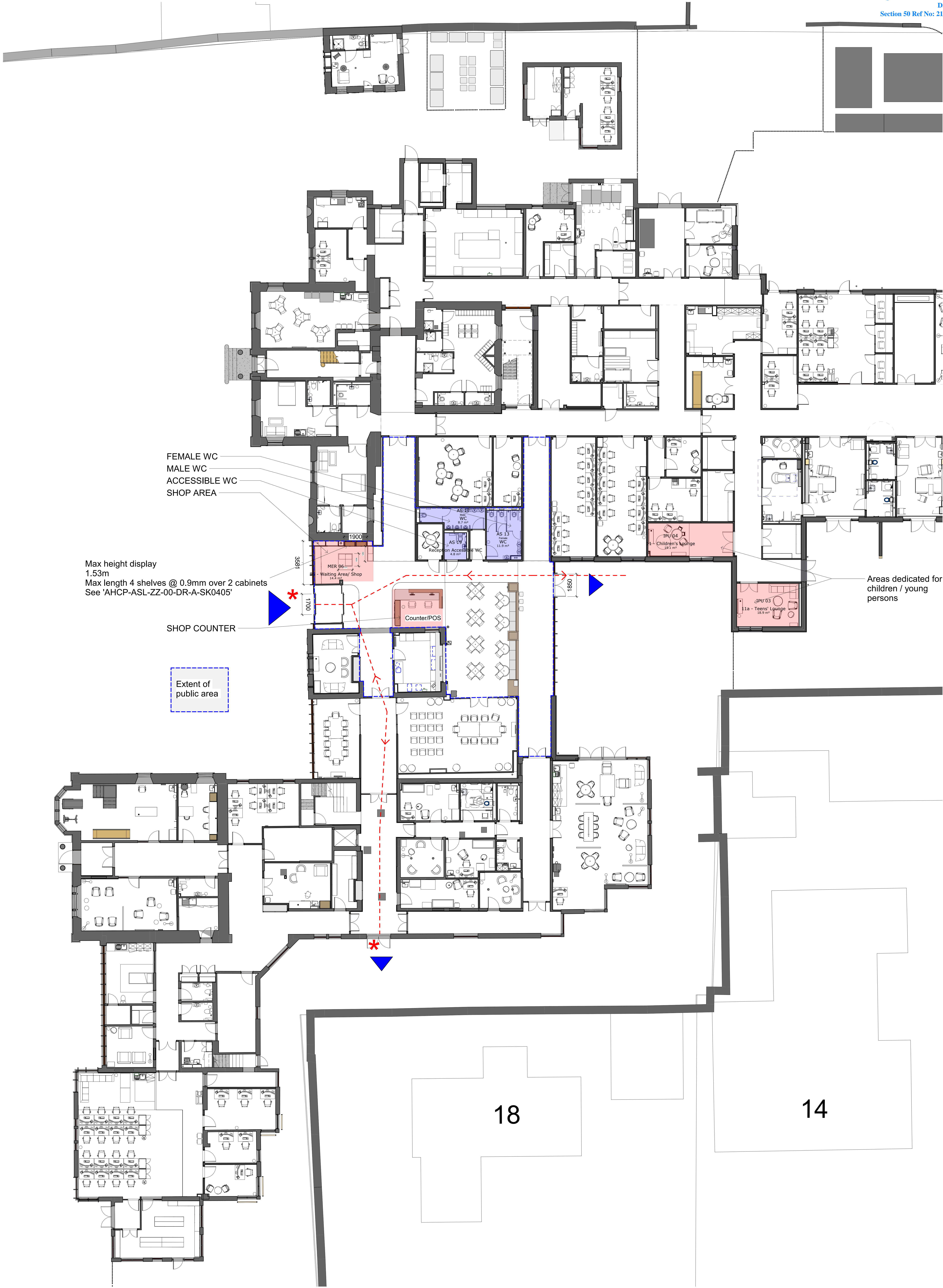
1 00 GA Ground Floor Proposed Licensing Plan 1 : 100
