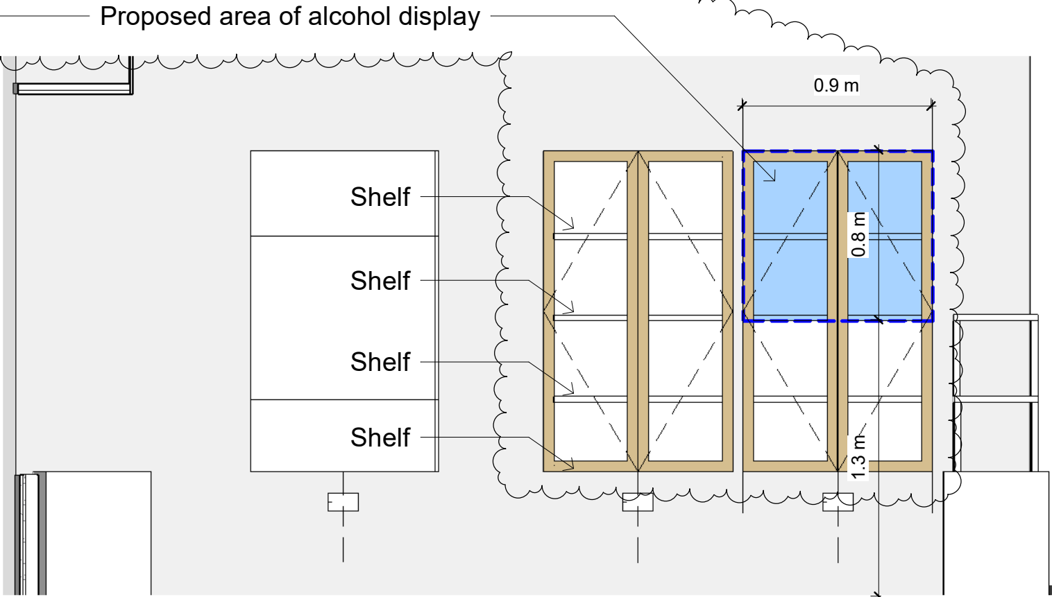
2 Licensing plans - Waiting Area / Shop - Display Elevation 1 : 25
