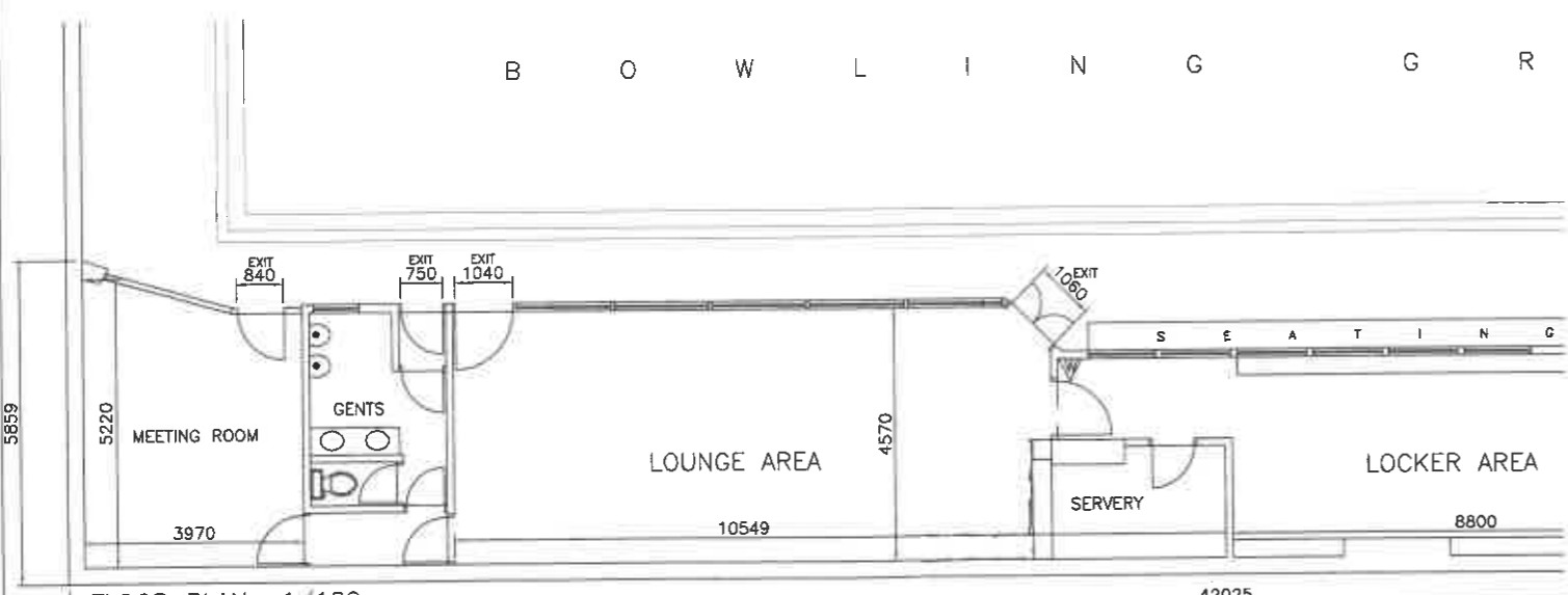
FLOOR PLAN 1/100
