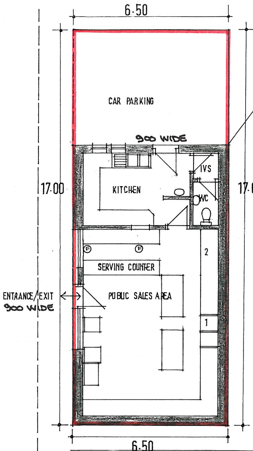
EXISTING PLAN 1: 100
