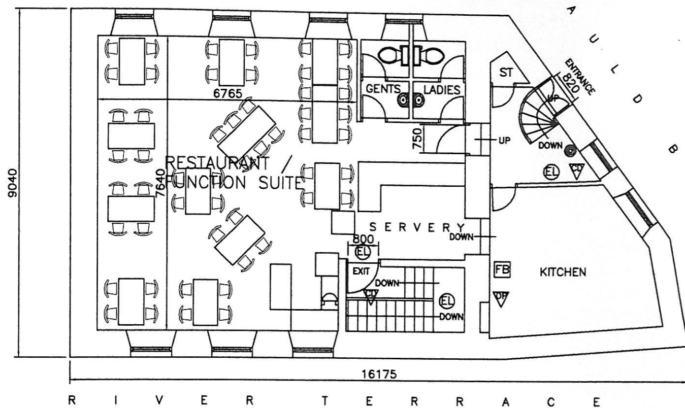
UPPER GROUND FLOOR PLAN 1/100
