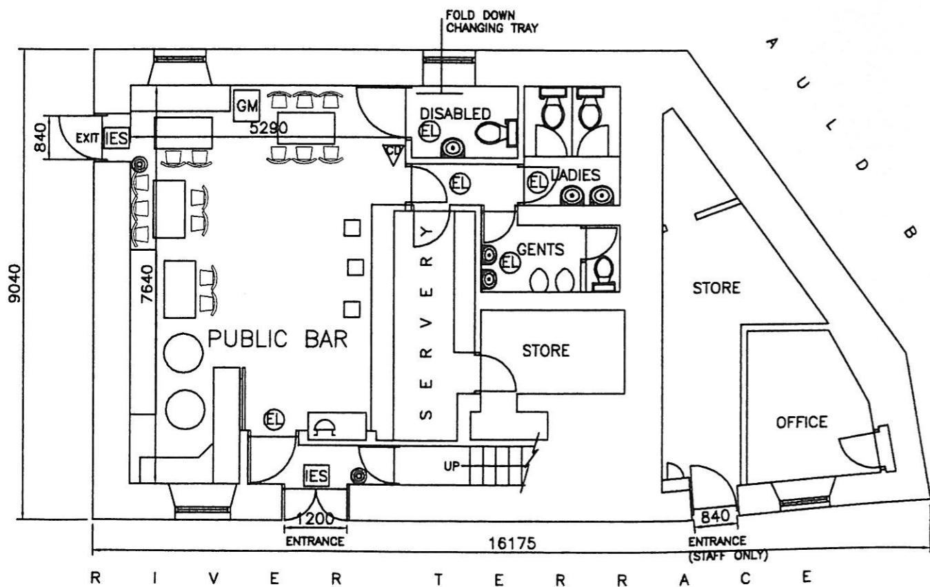
UPPER GROUND FLOOR PLAN 1/100
