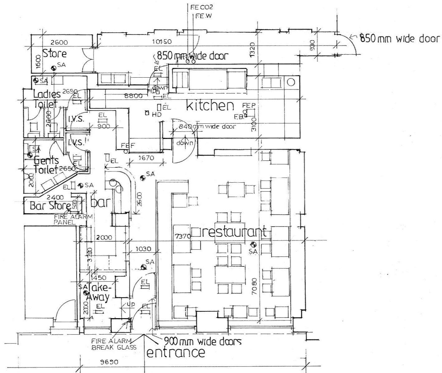
LAYOUT PLAN 1:100
