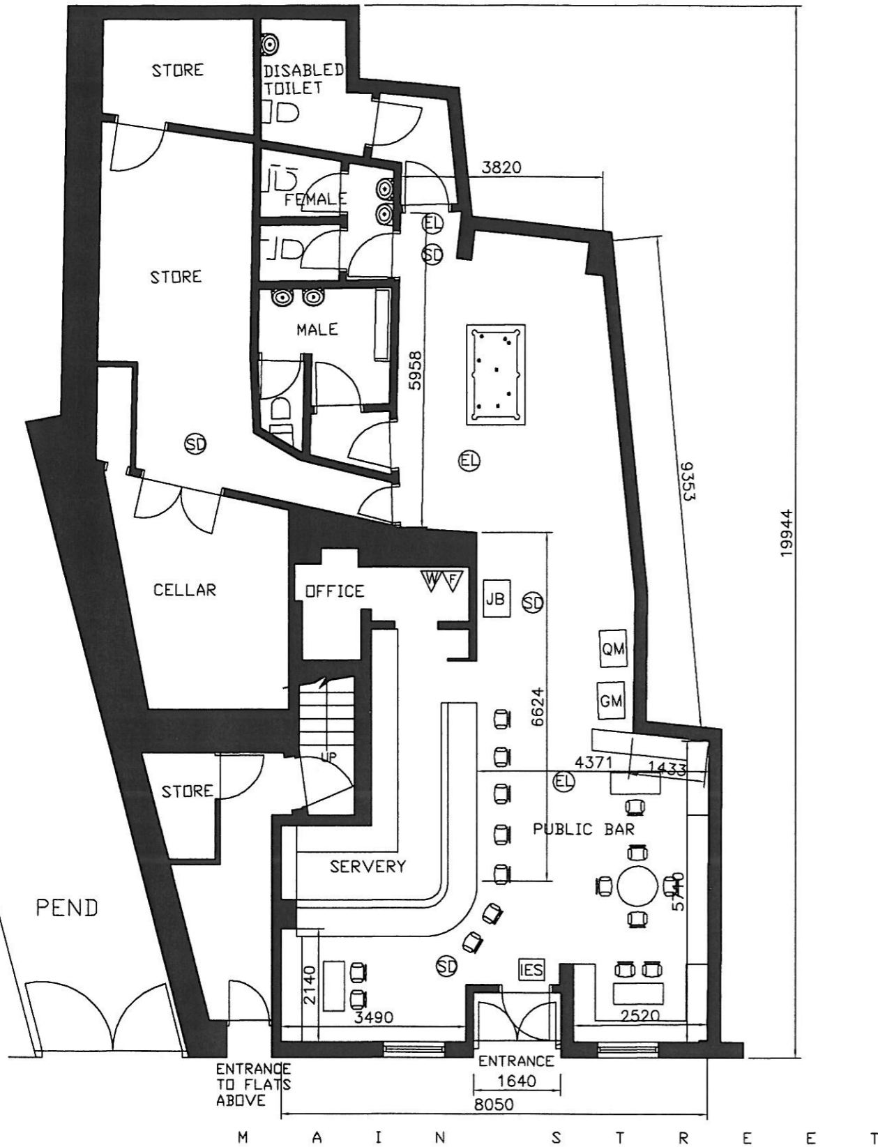
EXISTING FIRST FLOOR PLAN 1/100
