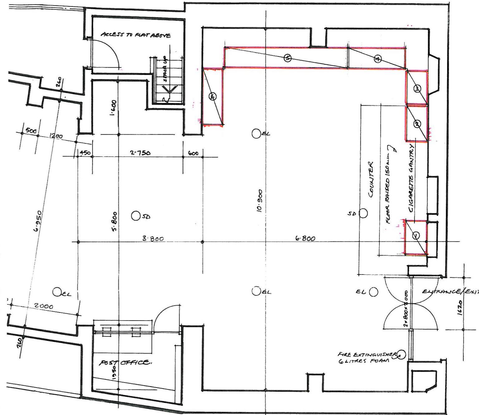
FLOOR PLAN OF SHOP AT 59 MONTGOMERIE STREET, TARBOLTON. SCALE 1:50.
