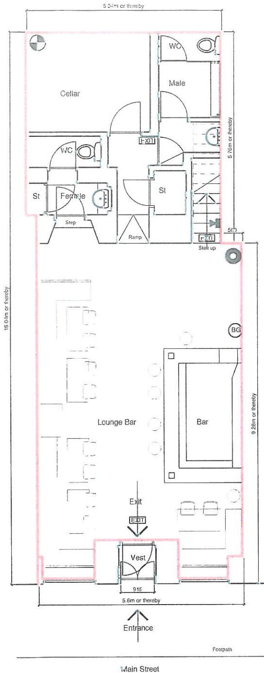
Ground Floor Plan Scale 1/100 metric
