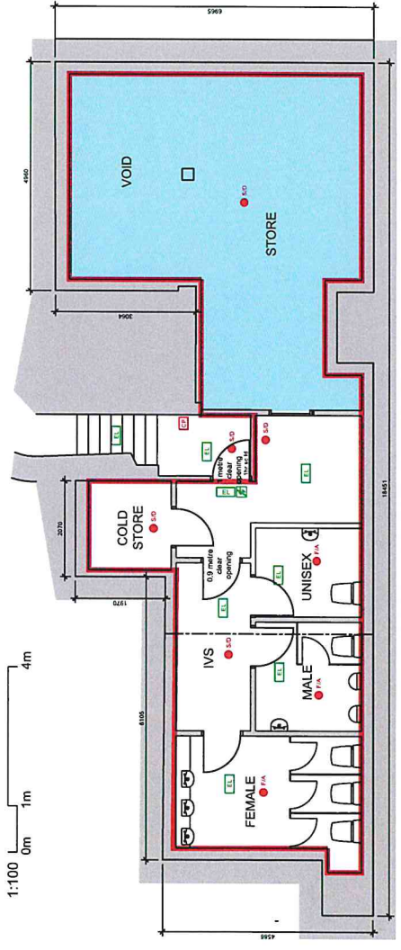
BASEMENT FLOOR PLAN 1:100 0m 1m 4m
